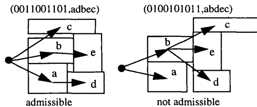
Figure 3: Admissible o-tree
