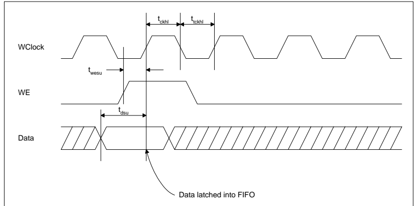
Figure 13-10. FIFO Write Cycle
