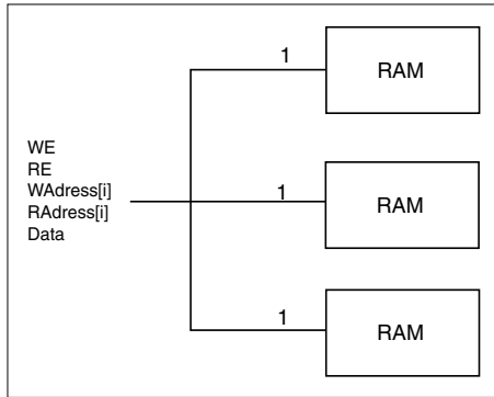
Figure 13-2. Manual Buffering (96x8 RAM Configuration)
